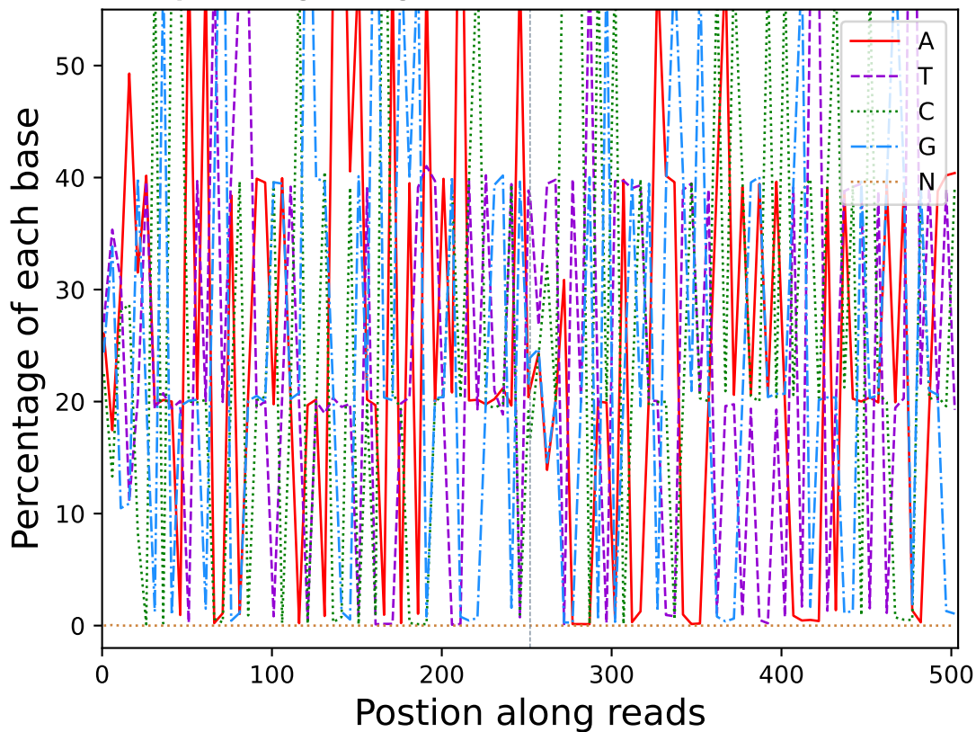
Base percentage along reads (R20102)
